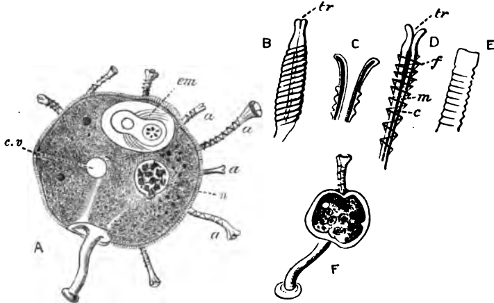
FIG. 62.— Choanophrya infundibulifera . A, adult; B-D, tentacles in action in various stages; E, tentacle at rest; F, young, just settled down. a, a, a , Tentacles in various stages of activity; c , central cavity; c. v. , contractile vacuole; em , ciliated embryo showing contractile vacuole and nucleus; f , spiral ridge; m , muscular wall of funnel; n , nucleus; tr , opening of funnel. (A-D, F, modified after Zenker; E, original.)
